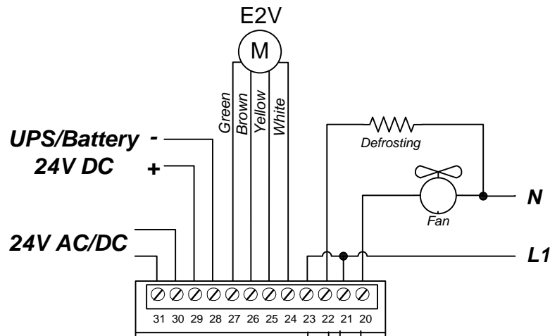
Figure 3.10.2 DC34D E2V
