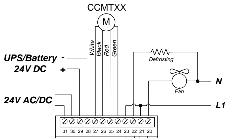
Figure 3.10.3 DC34D CCMT4
