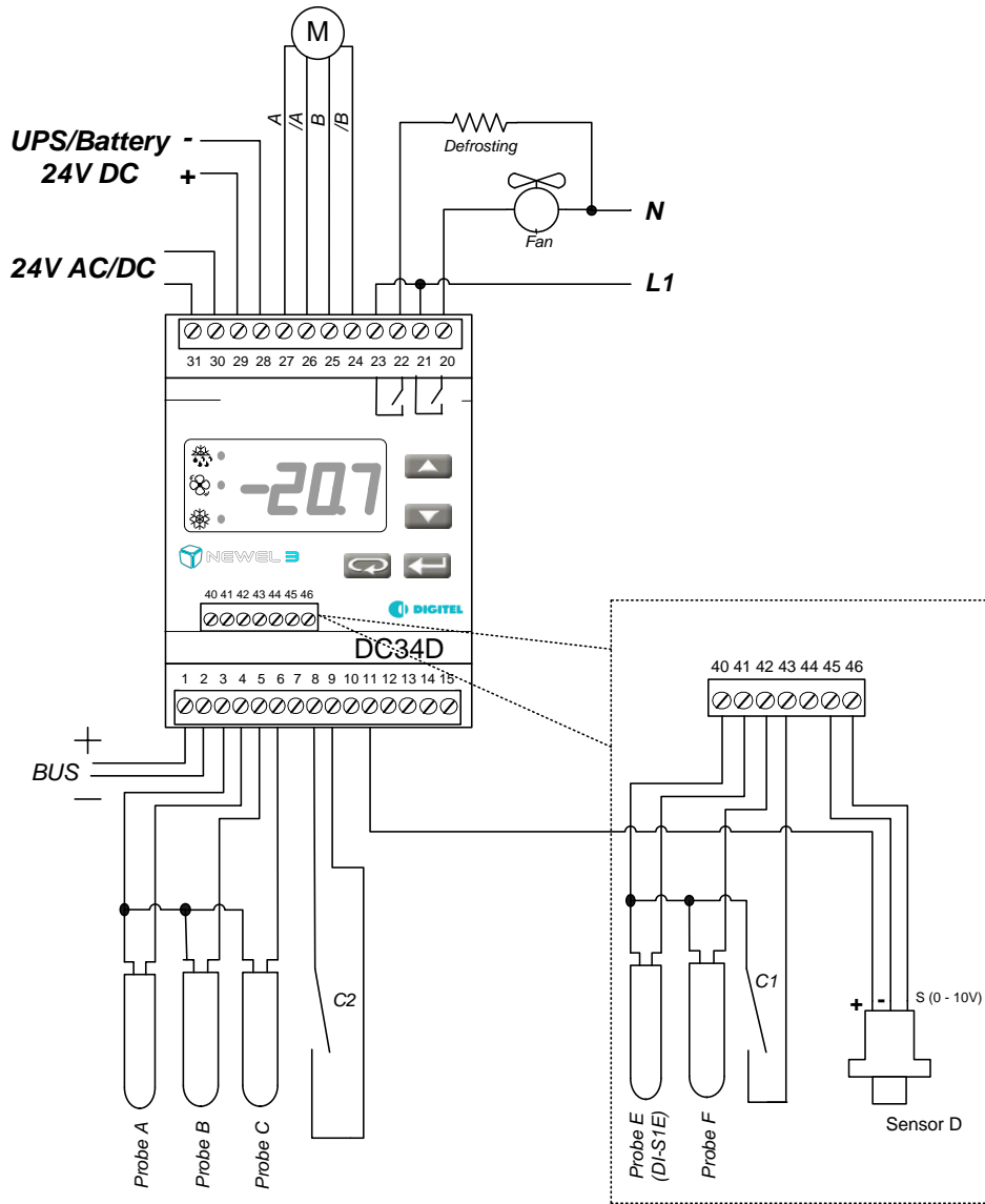
Figure 3.10.1 DC34D
